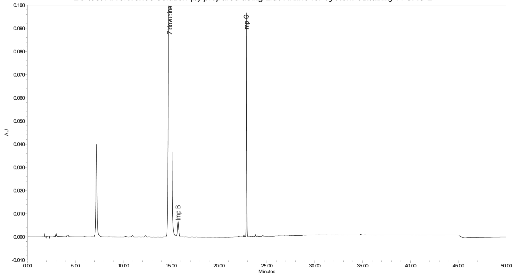
LC test A: reference solution (b) prepared using zidovudine for system suitability A CRS 2
