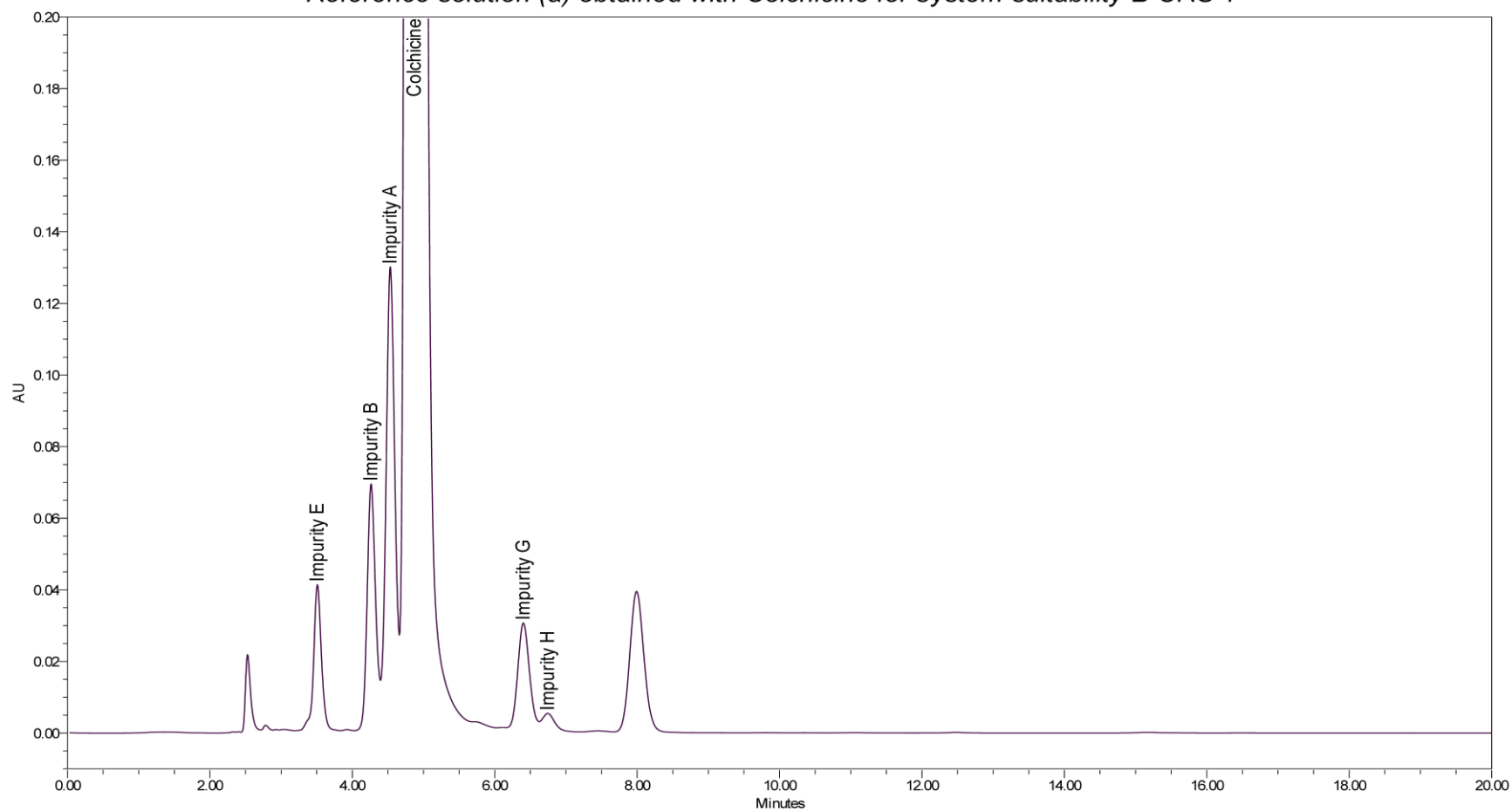
Reference solution (a) obtained with Colchicine for system suitability B CRS 1
